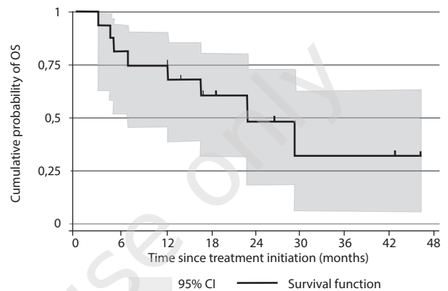
FIGURE 5. Kaplan–Meier curve for overall survival.
