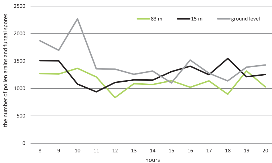
Figure 4. Hourly pollen and spore course at various heights (hours in summer time 8 = 06 UTC).
